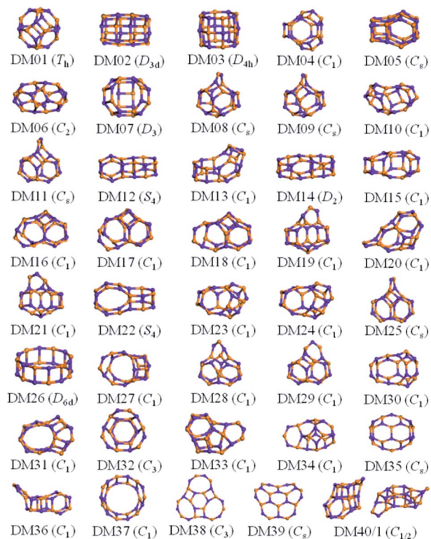
Fig. 7 ( \text{GaAs} ) 12 IP-LM configurations obtained by relaxing the DM-set of unique LM found by data-mining from other 1 : 1 compounds. Purple and orange atoms represent Ga and As, respectively, and the symmetry point groups of the clusters are given within parentheses.
