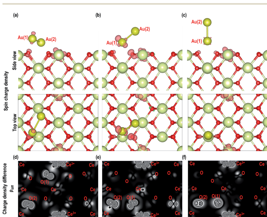
Fig. 12 Top and side view of isosurface ( 0.007 e \text{ \AA}^{-3} ) of spin densities of \text{Au}_2 on \text{CeO}_2(110) surface for (a) M_{\text{Au-Dim } 1} , (b) M_{\text{Au-Dim } 2} and (c) M_{\text{Au-Dim } 3} and 2D charge density difference contour maps of (d) M_{\text{Au-Dim } 1} , (e) M_{\text{Au-Dim } 2} and (f) M_{\text{Au-Dim } 3} .
