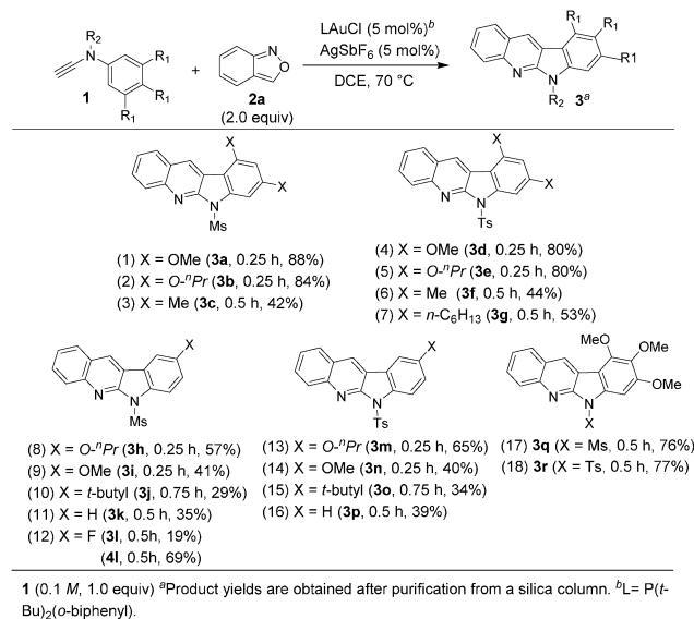
Scheme 1 Catalytic annulations with various N -arynylamides.
