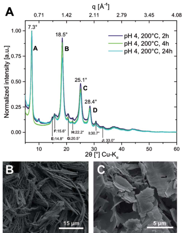
Fig. 3 Crystallinity of hydrothermally prepared PI6. (A) PXRD pattern of PI6 prepared at 200^\circ\text{C} and pH = 4 at t_{\text{h}} = 2 \text{ h} (dark blue); 4 h (green) and 24 h (turquoise). Reflections are labelled (A)–(J) with annotated scattering angles 2\theta (Cu-K \alpha ). (B) SEM image of PI6 synthesized at 200^\circ\text{C} and pH = 4 for 24 h. (C) SEM image of PI6 synthesized at 200^\circ\text{C} and pH = 1 for 24 h.
