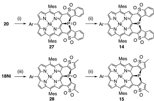
Scheme 3 Synthesis of (thiophene 1,1-dioxide)-fused porphyrins 14 and 15 (Ar = 3,5-di- tert -butylphenyl). (i) \text{H}_2\text{O}_2 , \text{Na}_2\text{WO}_4 \cdot 2\text{H}_2\text{O} , \text{MeN}(\text{C}_8\text{H}_{17})_3 \cdot \text{HSO}_4 , \text{PhPO}(\text{OH})_2 , toluene/ \text{H}_2\text{O} , 50 °C, 84%; (ii) \text{HSiCl}_3 , toluene, 110 °C, ( 14 : 26%, 15 : 28%); (iii) \text{H}_2\text{O}_2 , \text{Na}_2\text{WO}_4 \cdot 2\text{H}_2\text{O} , \text{MeN}(\text{C}_8\text{H}_{17})_3 \cdot \text{HSO}_4 , \text{PhPO}(\text{OH})_2 , toluene/ \text{H}_2\text{O} , 70 °C, 43%.
