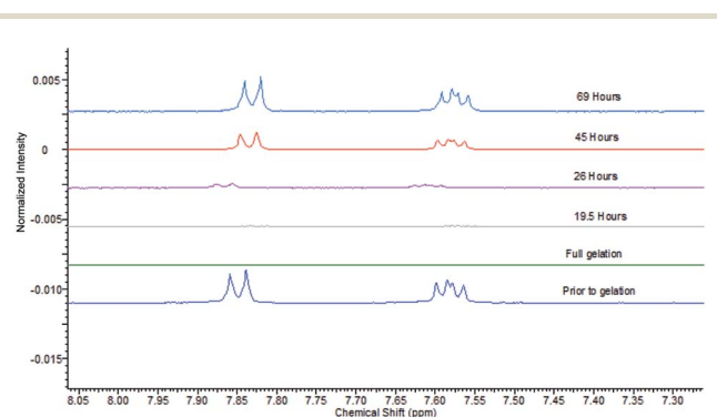
Fig. 8 NMR spectra of aromatic protons of DBS-COO 2 H (0.2% wt/vol), agarose (0.5% wt/vol) and heparin (1 mM), (from bottom to top) prior to gelation, after full gelation, and after various times (19.5 h, 26 h, 45 h and 69 h) of exposure to NaOH.
