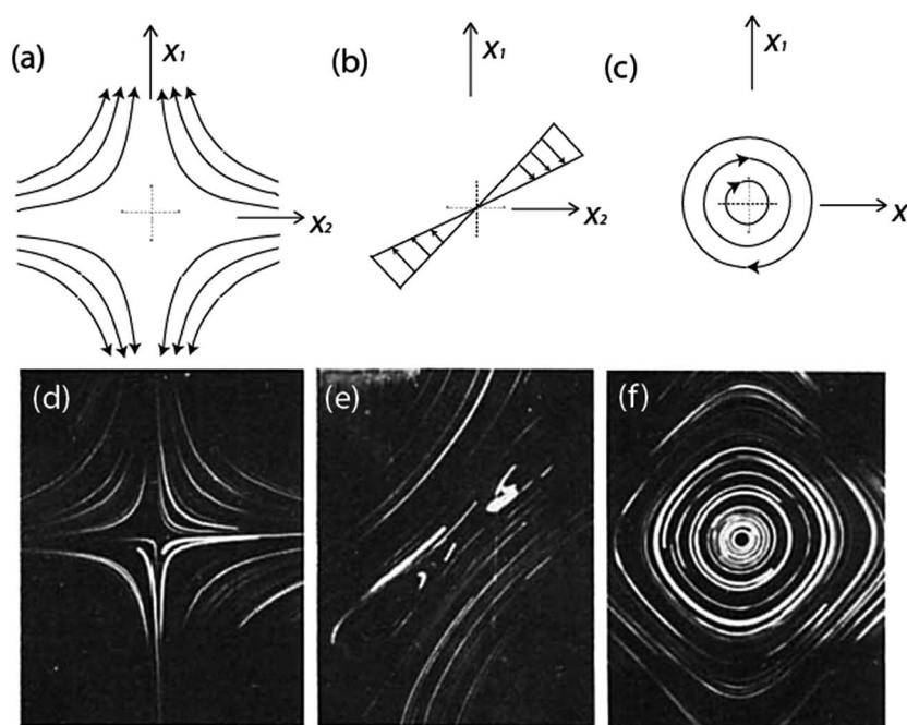
Fig. 2 Streamline schematics of stagnation point flow fields. (a) Extensional flow ( \lambda = 1 ). (b) Shear flow ( \lambda = 0 ). (c) Rotational flow ( \lambda = -1 ). Experimental captured photographs for stagnation point flow field. (d) \lambda = 1 . (e) \lambda = 0 . (f) \lambda = -1 . Type parameter varies from pure extensional flow to pure rotational flow. Reprinted with permission. Copyright© 1981 John Wiley & Sons, Inc. 31
