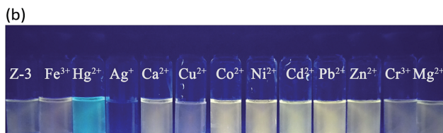
Fig. 1 (a) Fluorescence spectra ( \lambda_{\text{ex}} = 400 \text{ nm} ) of Z-3 ( 2 \times 10^{-5} \text{ M} ) with different metal ions: \text{Fe}^{3+} , \text{Hg}^{2+} , \text{Ag}^+ , \text{Ca}^{2+} , \text{Cu}^{2+} , \text{Co}^{2+} , \text{Ni}^{2+} , \text{Cd}^{2+} , \text{Pb}^{2+} , \text{Zn}^{2+} , \text{Cr}^{3+} and \text{Mg}^{2+} (10 equiv., respectively) in DMSO/ \text{H}_2\text{O} (v/v, 3 : 2; buffered with HEPES, pH = 7.20). (b) Visual fluorescence emission of the Z-3 sensor upon the addition of different metal ions.
