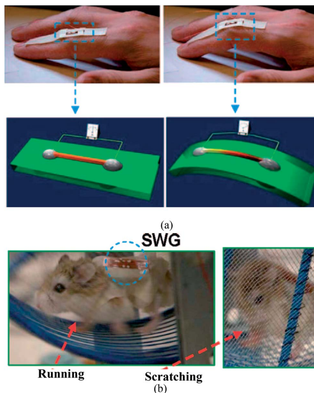
Fig. 20 Energy harvesting using an SWG from (a) an oscillating human index finger and (b) a live hamster. 8
