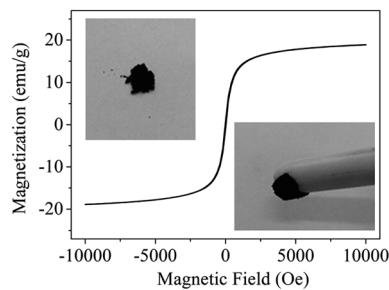
Fig. 6 Magnetization curve of the magnetic PPy-GO.
