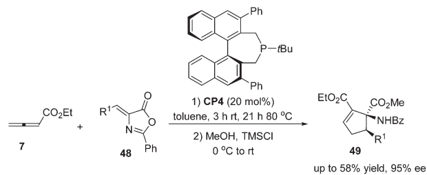
Scheme 16 The catalytic asymmetric Lu's [3 + 2] cycloadditions of allenic phosphonates with olefinic azalactones.
