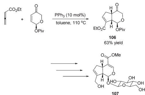
Scheme 34 Total synthesis of (+)-geniposide.
