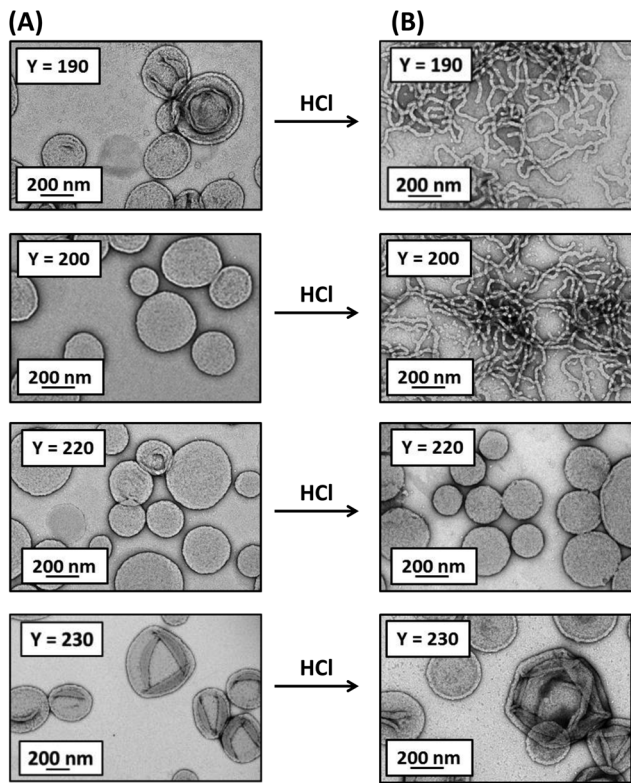
Fig. 2 Transmission electron microscopy images obtained for 0.1% w/w aqueous dispersions of MPETTC-PGMA 43 -PHPMA \gamma ( \gamma = 190, 200, 220 and 230 ) diblock copolymer nanoparticles at either (A) pH 7.0 or (B) pH 3.0. The pH switch was performed at 20 °C at 10% w/w copolymer concentration in each case.
