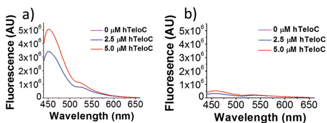
Fig. 1 Fluorescence emission of TO (5 μM) in the presence of 0–5 μM hTeloC in 10 mM sodium cacodylate buffer at pH 5.5 (a) and pH 7.4 (b).
