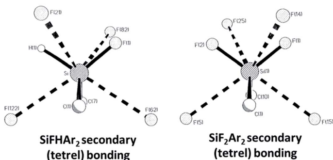
Fig. 11 Crystal structure of SiFHA 2 , Ar = C 6 H 2 (CF 3 ) 3 (top), with secondary (tetrel) bonding shown as dashed bonds. Primary bonding (solid lines) and secondary bonding (dashed lines) at Si in SiFHA 2 and SiF 2 Ar 2 (bottom). Secondary (tetrel) Si···F bonds are longer than primary (covalent) Si–F bonds. Secondary bonds trans to F are shorter than those trans to C. Adapted from ref. 57 with permission from Elsevier.
