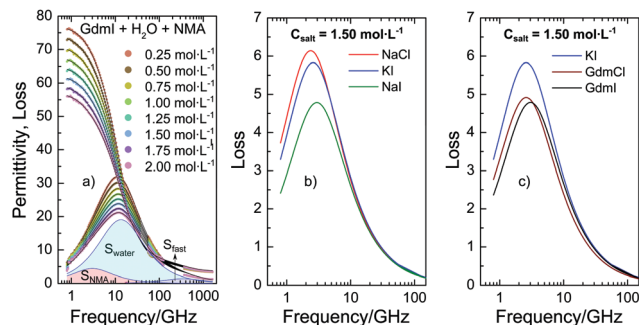
Fig. 1 (a) Complex permittivity spectra of binary mixtures of water and NMA ( 2 \text{ mol L}^{-1} ) with increasing Gdml concentration. The shaded areas correspond to contributions of bulk water, NMA, and fast water to the dielectric loss for c_{\text{salt}} = 2 \text{ mol L}^{-1} Gdml. The symbols correspond to the experimental data, while the solid lines to fits with eqn (1). The Ohmic loss (last term of eqn (1)) has been subtracted for visual clarity. (b and c) Dielectric loss due to NMA as obtained from fitting eqn (1) to the experimental spectra (imaginary part of the first term of eqn (1)) for samples containing 2 \text{ mol L}^{-1} NMA and c_{\text{salt}} = 1.5 \text{ mol L}^{-1} salt for different salts. Data for NaCl, KI, and GdmCl were taken from ref. 19–21.
