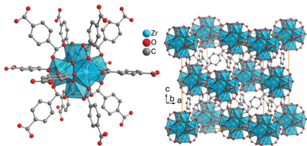
Fig. 9 Structure of zirconium terephthalate UiO-66Zr. The SBU is a hexanuclear and octahedral cluster of six edge-sharing \text{ZrO}_6 square antiprisms, which is connected to 12 neighboring SBUs in a face-centered cubic (fcc) packing arrangement. The structure was drawn from deposited cif-files under CCDC 837796 (UiO-66). 81
