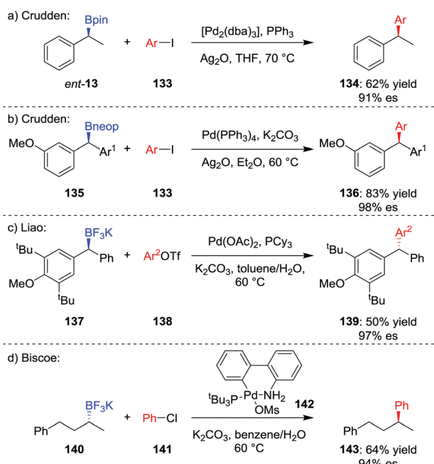
Scheme 19 Enantiospecific transition-metal-mediated sp^2 – sp^3 cross-coupling of unactivated secondary boronic esters and trifluoroborate salts. Ar = p\text{-}ClC_6H_4 , Ar^1 = p\text{-}CH_3CH_2C_6H_4 , Ar^2 = p\text{-}CH_3C_6H_4 , Ms = CH_3SO_2 , neop = neopentyl glycol.
