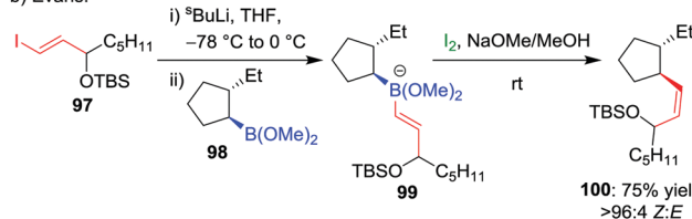
Scheme 14 Early examples of the Zweifel olefination reaction applied to boranes and boronic esters.
