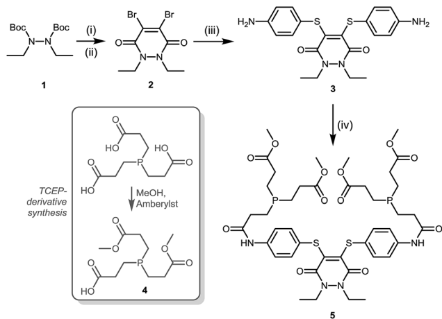
Scheme 1 Synthesis of dithioaryl(TCEP)pyridazinedione 5 . Reagents and conditions: (i) TFA, \text{CH}_2\text{Cl}_2 , 21 °C, 1 h; (ii) dibromomaleic anhydride, AcOH, reflux, 2 h; (iii) 4-aminothiophenol, \text{NEt}_3 , \text{CH}_2\text{Cl}_2 , 21 °C, 2 h; (iv) acid 4 , DMF, HATU, DIPEA, 21 °C, 12 h.
