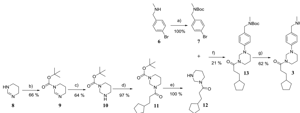
Fig. 4 Synthetic scheme for the preparation of 3-cyclopentyl-1-(3-(4-(methylamino) methyl)phenyl) tetrahydropyrimidin-2(1H)-yl)propan-1-one (3). (a) di- tert -butyl dicarbonate, NEt 3 , THF; 0 → 22 °C; overnight; (b) di- tert -butyl dicarbonate, NEt 3 , THF; 0 → 22 °C; overnight; (c) NaBH 4 , MeOH, 0 °C; 2 h; (d) 3-cyclopentylpropionic acid, DCM, diisopropylethylamine, COMU, 22 °C; 18 h; (e) TFA, DCM, 22 °C; 2 h; (f) Pd(OAc) 2 , KO t Bu, 2-(di- tert -butylphosphino) biphenyl, toluene; 100 °C, 4 h; (g) TFA, DCM, 22 °C; 2 h.
