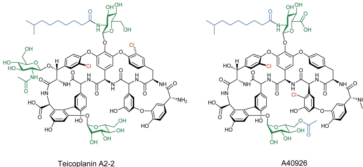
Fig. 9 Structures of teicoplanin A2-2 and the related A40926. Glycosylation sites heightened in green and acylation sites in blue. 39,40
