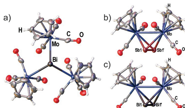
Fig. 2 (a) Crystal structure of [(CpMo(CO) _3 ) _3 Bi] (4) with viewing direction along the threefold symmetry axis. (b) Crystal structure of the \text{Sb}_2 complex 3c. (c) Crystal structure of the \text{Bi}_2 complex 3d. Selected bond lengths [Å] and angles [°]: 4: Mo–Bi 3.014(3), angle Mo–Bi–Mo = 113.50(5)°. 3c: Mo1–Mo1' 3.1183(10), Sb1–Sb1' 2.6871(7). 3d: Mo1–Mo1' 3.1378(13), Bi1–Bi1' 2.8580(7). Ellipsoids are drawn at 50% probability for 3c,d and 30% probability for 4.
