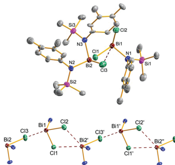
Fig. 5 ORTEP drawing of the molecular structure of 5e/9e (top) and representation of the chain-like structure in the crystal of 5e/9e (bottom, view along a -axis). Thermal ellipsoids with 50% probability at 173 K (hydrogen atoms omitted for clarity). Selected distances (Å) and angles ( ^\circ ): Bi1–Cl1 2.4702(2), Bi1–Cl2 2.550(2), Bi2–Cl3 2.581(2), Bi1–N1 2.116(6), Cl2–Bi1–Cl3 171.000(6), Cl1–Bi1–Cl3 83.360(7); long range distances: Bi1–Cl3 3.057(2), Bi2'–Cl1 3.516(2), Bi2'–Cl2 3.644(2), Bi1–Bi2 4.8481(3).
