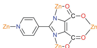
Fig. 12 Section of the structure of [Zn_2(pidc)(H_2O)Cl]_n . 78
