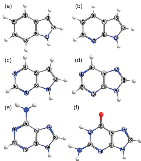
Fig. 2 Bicyclic molecules considered in this work: (a) indole, (b) 7-azaindole, (c) 5,7-azaindole, (d) 9 H -purine, (e) adenine (A) and (f) guanine (G), with the ring atoms numbered for future reference.
