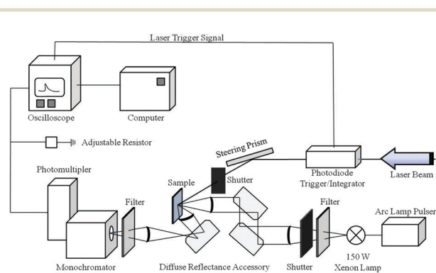
Fig. 1 Schematic diagram of the nanosecond diffuse reflectance laser flash photolysis apparatus to produce and detect transient absorptions in light-scattering samples.
