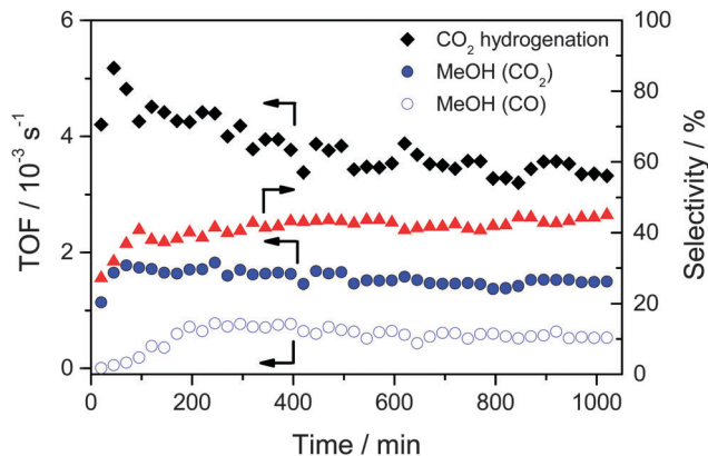
Fig. 2 Time dependent MeOH formation activity (TOF) of the Au/ZnO catalyst (STEM Chemicals) during CO 2 hydrogenation (●, 15% CO 2 /45% H 2 /balance Ar) and CO hydrogenation (○, 15% CO/45% H 2 /balance Ar) at 5 bar and 240 °C after calcination in 1% O 2 /Ar at 20 Nml min -1 and 400 °C for 1 h (O400). For CO 2 hydrogenation the activity (TOF) (◆) and selectivity (▲) for MeOH formation are also included.
