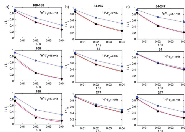
Fig. 2 Prototypical ^1\text{H}^{\text{N}}-\Gamma_2 relaxation measurements for residues displaying negative (a), vanishing (b) or positive (c) dipole–dipole cross-correlation effects. ^1\text{H}^{\text{N}} data are shown for residues 125 of C108–C188 (a), 115 of C54–C247 (b) and 227 of C54–C247 (c) in doubly spin labeled (top) and the corresponding singly labeled OPN mutants (black: active MTSL, blue: reduced MTSL). The obtained ^1\text{H}^{\text{N}}-\Gamma_2 relaxation rates are also given and were extracted by fitting the data to I/I_0 = \exp(-R_2t) (not shown). The obtained rates were in agreement with a model for transverse relaxation in AMX spin systems developed by Kay and Bull (purple fits, see the text).
