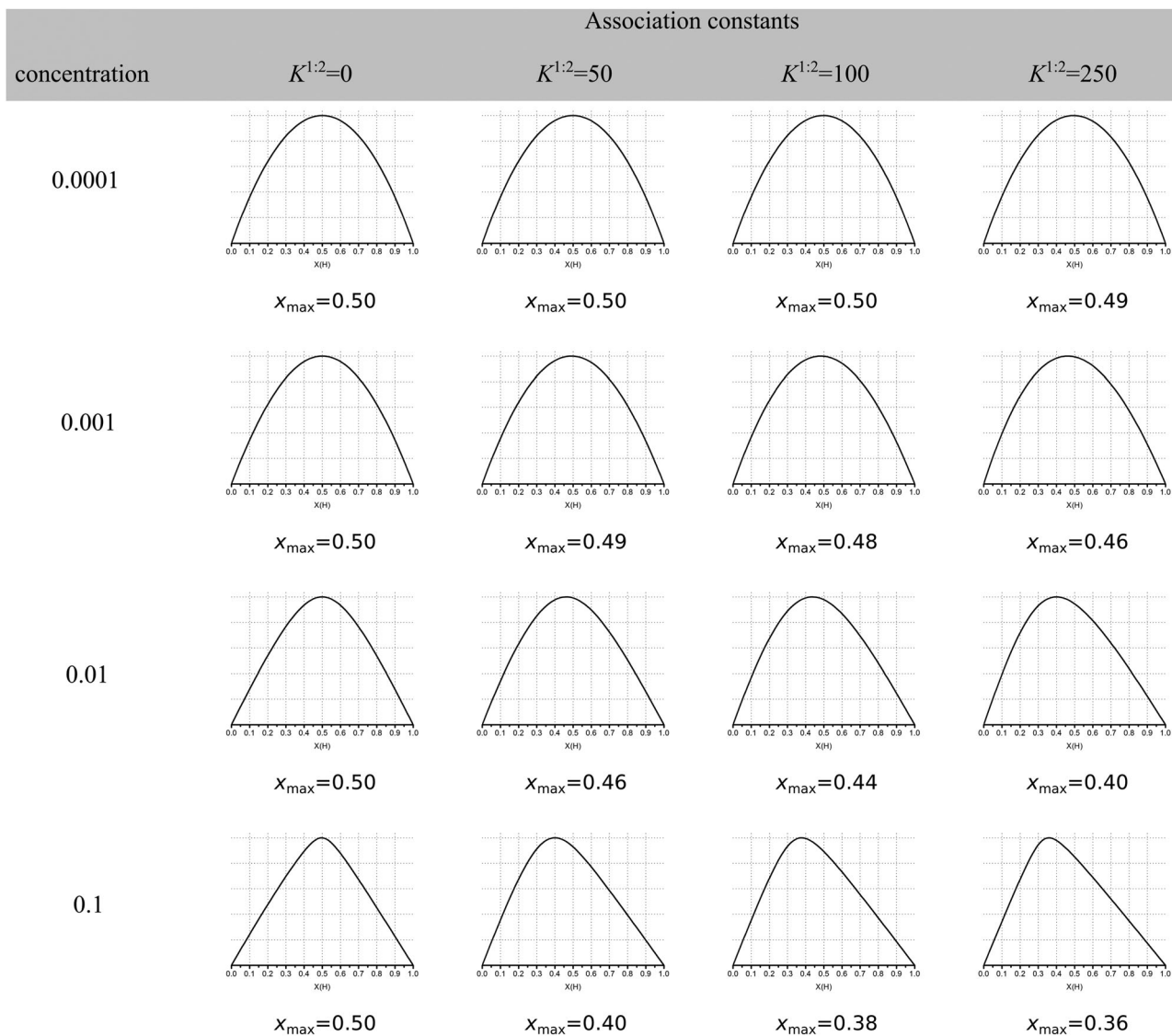
Fig. 1 Simulated Job Plots for various cases of 1:2 stoichiometry with the exception of the 1:1 complexes in column 2 ( K_2 = 0 ). In all cases K_1 = 1000 \text{ M}^{-1} with Y_{\text{HG}} = 1 and Y_{\text{HG}_2} = 2 (additive model). The concentration of host in M is shown in column 1. The simulated maxima in the Job plots is shown as x_{\max} . Reproduced with permission from ref. 16.
