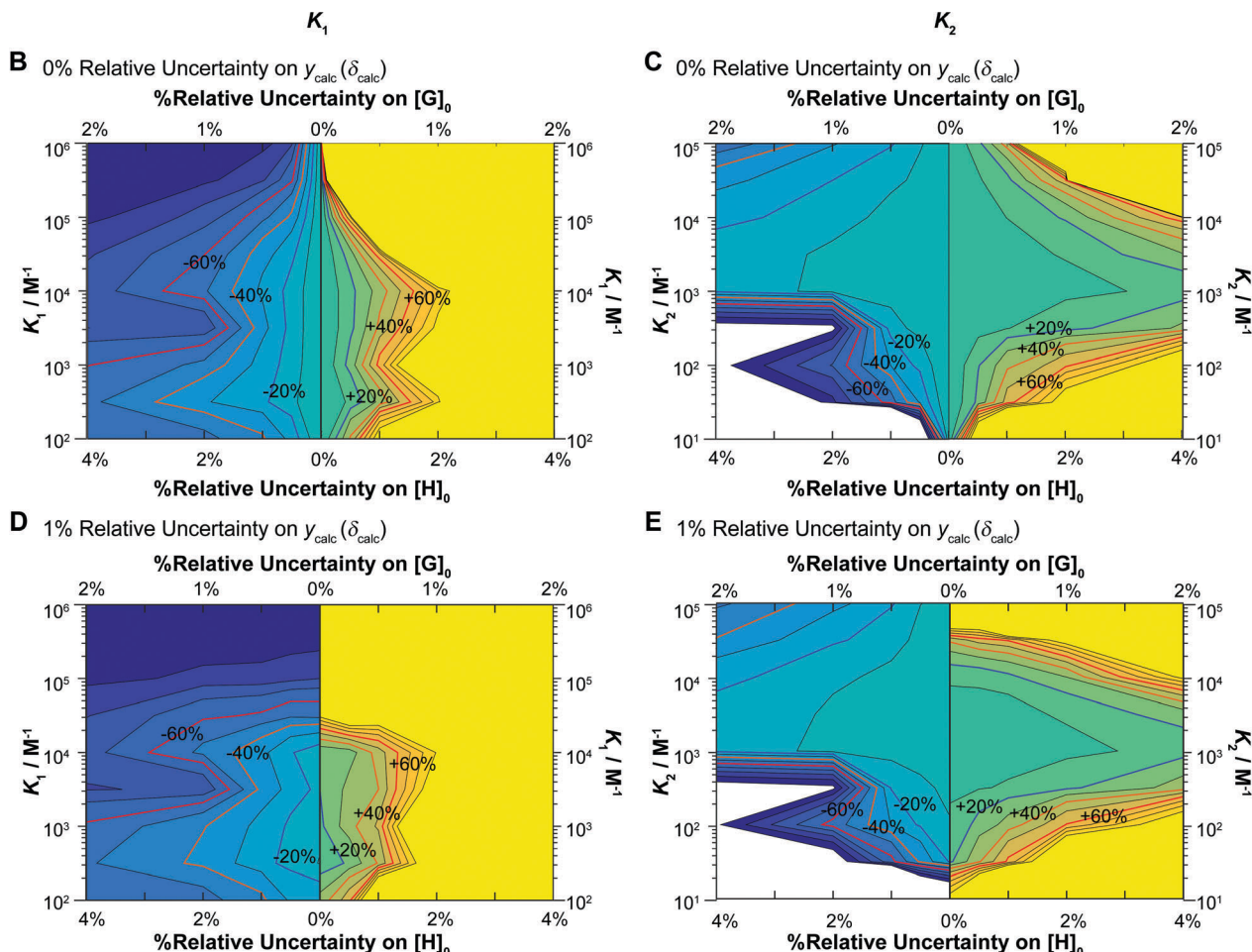
Fig. 6 Monte Carlo simulations ( M = 200 ) for NMR titrations with underlying 1 : 2 equilibria (full model). In all cases [H]_0 = 10^{-3} M, [G]_0 is spread unevenly across 49 data points between [G]_0 = 0-0.035 M, with \delta_{HG} = 0.5 ppm and \delta_{HG_2} = 1 ppm (as in the additive model – Fig. 3B) as the starting values in the “ideal” datasets used at the start of these simulations. The data was fitted with K_1 between 10^2-10^6 M ^{-1} and K_2 between 10-10^5 M ^{-1} with K_2 always fixed at K_2 = 0.1 \times K_1 (mild negative cooperativity). The variance is either 0% or 1% on y_{\text{calc}} ( \delta_{\text{calc}} ), 0–2% on [G]_0 and 0–4% on [H]_0 . In each case the variance of [H]_0 is 2 \times that of [G]_0 . The contour plot is coloured according to relative (%) the Monte Carlo uncertainty on the expected K_1 (left column) and K_2 (right column) values at the 95% confidence interval level (95% CI). (A) The colour scheme used in the contour plots between -100\% and +100\% of the expected K_1 or K_2 values. (B) Contour plot of the calculated Monte Carlo 95% CI on K_1 assuming uncertainty of 0% for y_{\text{calc}} ( \delta_{\text{calc}} ). The lines indicate steps of 10%. The \pm 20\% (blue) \pm 40\% (orange) and \pm 60\% (red) levels are highlighted with bold lines and labels. The y-axis represents changes in K_1 . Starting from the central vertical line, the x-axis represents increasing noises in [H]_0 and [G]_0 for the lower limit (left side panel) and higher limit (right side panel) of the expected K_1 . (C) Same as (B) except for K_2 instead of K_1 including the y-axis which shows K_2 . (D) Same as (B) except with additional 1% relative standard deviation on y_{\text{calc}} ( \delta_{\text{calc}} ). (E) Same as (D) except for K_2 instead of K_1 including the y-axis which shows K_2 . Note the order of magnitude difference in the y-axis between the left ( K_1 ) and right ( K_2 ) columns.
