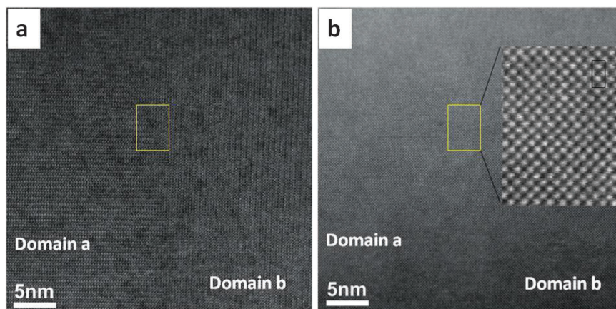
Fig. 7 (a) Aberration corrected bright field (BF) STEM image of the twin boundary, (b) corresponding HAADF of the twin boundary, the enlarged HAADF image of a part of twin boundary is shown in the right side of the image. The rectangle in each figure represents the unit cell.
