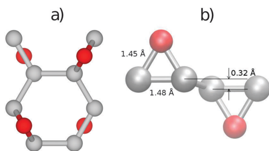
Fig. 1 (a) The top view of the 8-C and 4-O atom unit cell of the most stable structure of fully oxidized graphene and (b) the 60° relative to the x-axis side view of the epoxy groups formed by O atoms adsorbed on opposite sides of the graphene sheet, together with the C–C and C–O bond-lengths. The C and oxygen atoms are represented by grey and red spheres, respectively.
