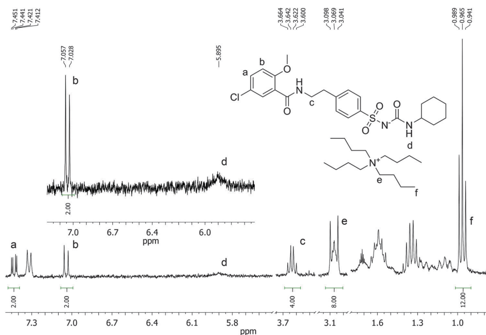
Fig. 6 ^1\text{H} NMR spectrum of the supernatant solution of NP (10 mg) following equilibration with a 2 mmol \text{L}^{-1} solution of GLIB in \text{CD}_3\text{CN} showing a 2 : 1 ratio of GLIB : TBA signals.
