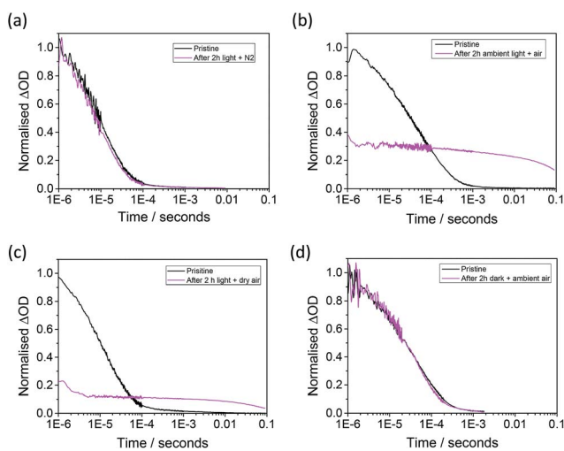
Fig. 4 Effect of exposure to varying environmental conditions for two hours on the transient absorption signal at 1600 nm for a mesoporous \text{Al}_2\text{O}_3/\text{MAPbI}_3/\text{spiro-OMeTAD} film: (a) ambient light, sealed under flowing \text{N}_2 , (b) ambient light, non-sealed, (c) ambient light, sealed under flowing dry air ( \text{H}_2\text{O} < 2 \text{ vpm} ), (d) dark, non-sealed. Laser excitation energy density = 25 \mu\text{J cm}^{-2} at 567 \text{ nm} .
