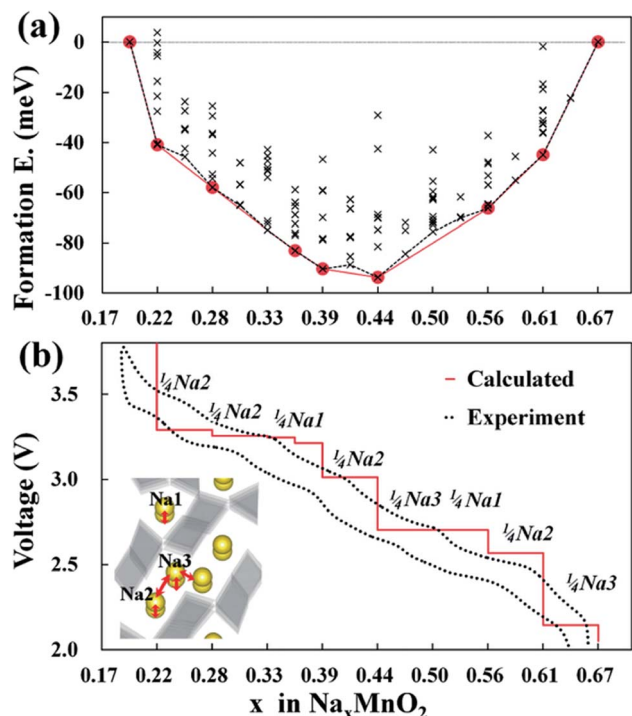
Fig. 6 (a) Formation energies of seven stable intermediate phases during \text{Na}_x\text{MnO}_2 cycling calculated from 156 different sodium configurations, and (b) experimental and calculated voltage profiles for \text{Na}_x\text{MnO}_2 with respect to the minimum energy path of formation energies. Reproduced with permission 35 © 2012, ACS Publications.
