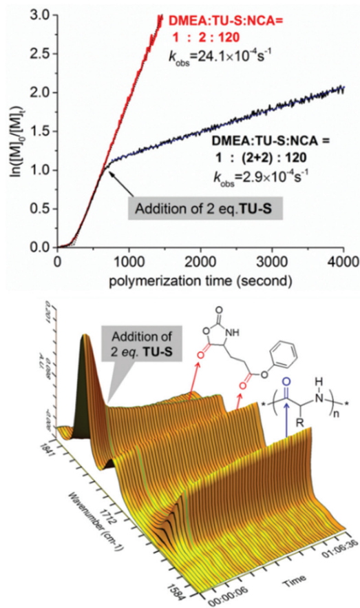
Fig. 6 \ln([NCA]_0/[NCA]_t) vs. time for the ROP of Glu-NCA initiated by DMEA/TU-S ( [M] = 0.19 M, [Glu-NCA]/[TU-S]/[DMEA] = 120/(2 + 2)/1 , 25 °C, \text{CH}_2\text{Cl}_2 ) and corresponding 3D kinetic behavior profile from in situ IR (the sampling interval of in situ IR is 10 seconds).
