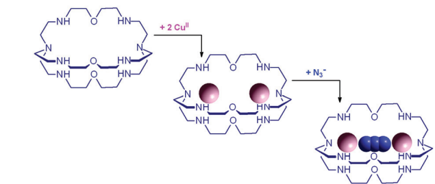
Fig. 1 Cascade process for the consecutive inclusion of two \text{Cu}^{\text{II}} ions, then of one azide anion into the bistren cryptand 2, to form the ternary dimetallic complex [\text{Cu}^{\text{II}}_2(2)(\text{N}_3)]^{3+} . Each terminal atom of the ambidentate anion establishes a coordinative interaction with a coordinatively unsaturated \text{Cu}^{\text{II}} centre bound to each tren subunit.
