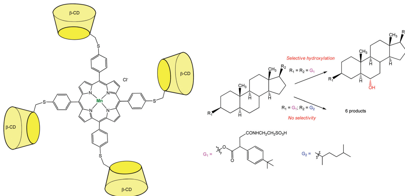
Fig. 10 Highly selective Mn-porphyrin catalyst based on a β-CD tetramer for steroid hydroxylation. 19
