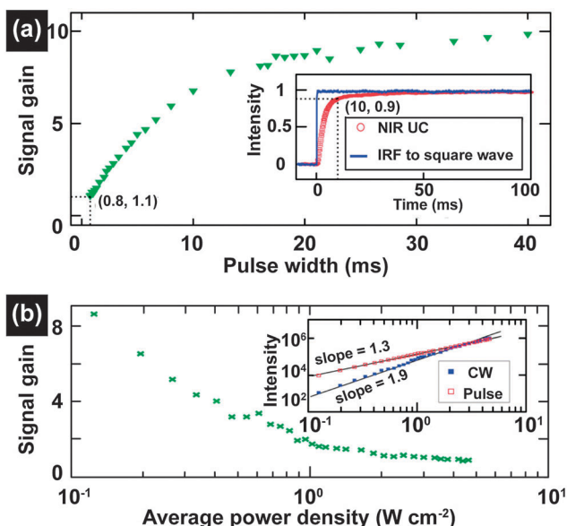
Fig. 16 Study of photon UC of lanthanide-doped nanocrystals under excitation of a millisecond single pulse. (a) The NIR UC signal gain of NaYF 4 :Yb/Tm (25/0.3 mol% )@NaYF 4 core-shell nanocrystals upon pulse excitation with different pulse widths (IRF—the instrument response function). (b) The dependence of NIR UC signal gain on the average power density under excitation of pulse-laser (pulse width, 20 ms; repetition rate, 2 Hz). Insets: the response of the NIR UC emission to a square-wave excitation (inset a) and the average power density dependences of the NIR UC emission intensity under CW and pulsed excitations (inset b), respectively. (Reprinted with permission from ref. 203. Copyright 2013, Royal Society of Chemistry.)
