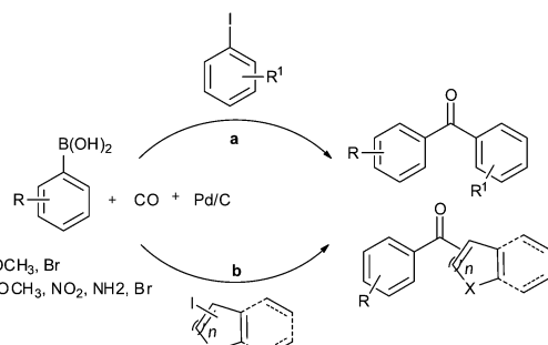
Scheme 45 Reagents and conditions: (a) aryl iodide (1 mmol), arylboronic acid (1.2 mmol), CO (200 psi), 10% Pd/C (2 mol%), K 2 CO 3 (3 mmol), anisole (10 mL), 100 °C, 8 h; (b) heteroaryl iodide (1 mmol), arylboronic acid (1.2 mmol), CO (200 psi), 10% Pd/C (2.5 mol%), K 2 CO 3 (3 mmol), toluene (10 mL), time 10 h, temp. 100 °C.
