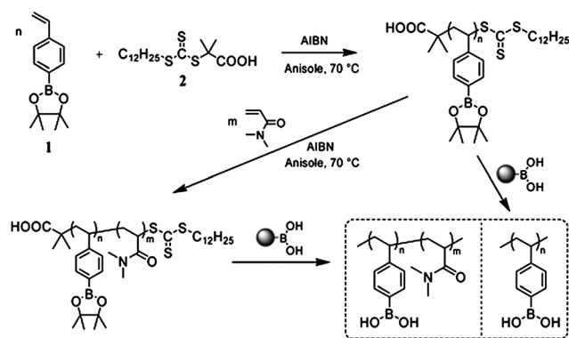
Fig. 8 Synthesis of boronic ester and boronic acid homopolymers and block copolymers by RAFT polymerization. (Reprinted with permission from ref. 45. Copyright © 2007, American Chemical Society.)
