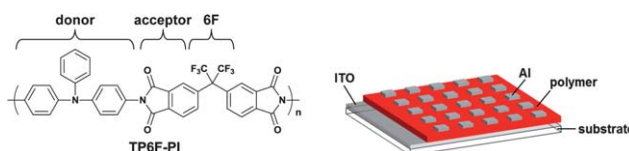
Fig. 2 The chemical structure of TP6F-PI and a schematic diagram of a polymer memory device.
