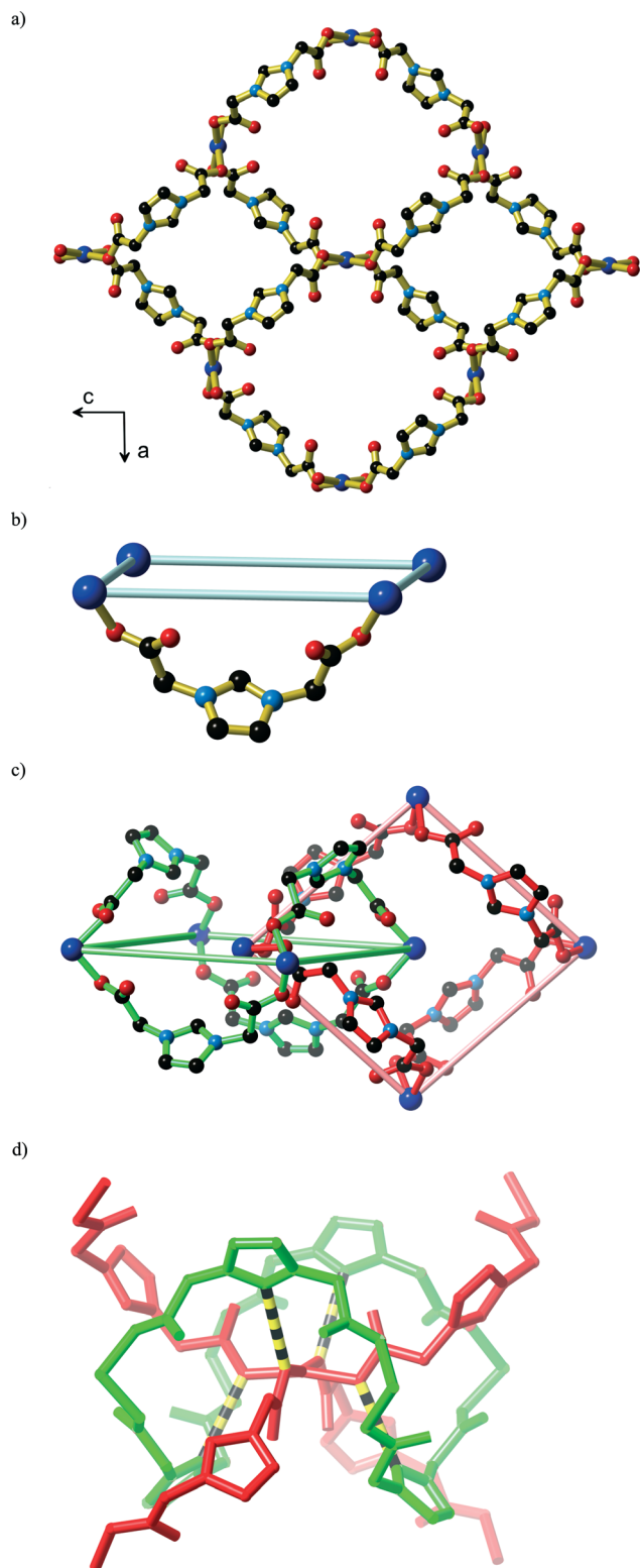
Fig. 6 The structure of \text{Cu}_2(\text{imdc})_2\text{NaBF}_4 \cdot 7\text{H}_2\text{O} (5) showing a) part of the 2D \text{Cu}(\text{imdc})_2 network with the two types of rhombic holes b) four \text{Cu}(\text{I}) centres which are linked by \text{imdc}^- ligands, that loop either above or below the plane of the \text{Cu}(\text{I}) centres; only one of the four \text{imdc} ligands is indicated c) two catenating rings, one from one sheet (red connections) the other from the perpendicular sheet (green connections) d) part of one framework (red connections) passing through one of the congested rings of a perpendicular framework (green connections); \text{C-H}\cdots\text{O} hydrogen bonds extending from the imidazolium groups of the green framework to coordinated oxygen atoms of the red framework are indicated by yellow and black striped connections.
