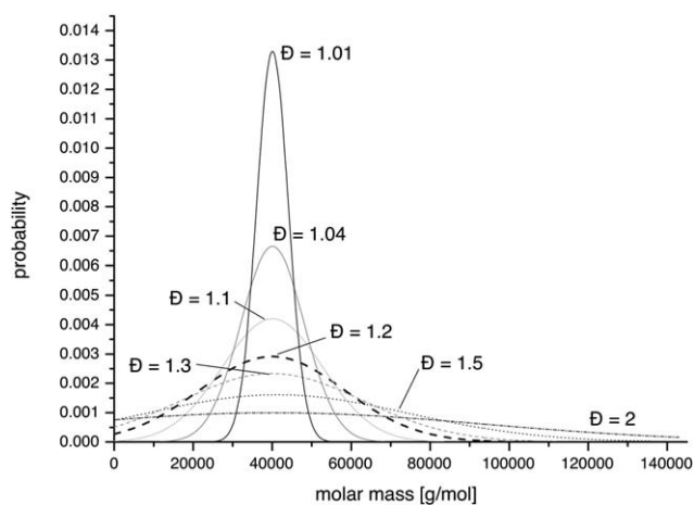
Fig. 2 Representation of theoretical Gaussian distributions of PHPMA with a degree of polymerisation of 30 ( M_n = 40 kg mol -1 ) with a variation in the dispersity from 1.01, 1.04, 1.1, 1.2, 1.5 to 2.
