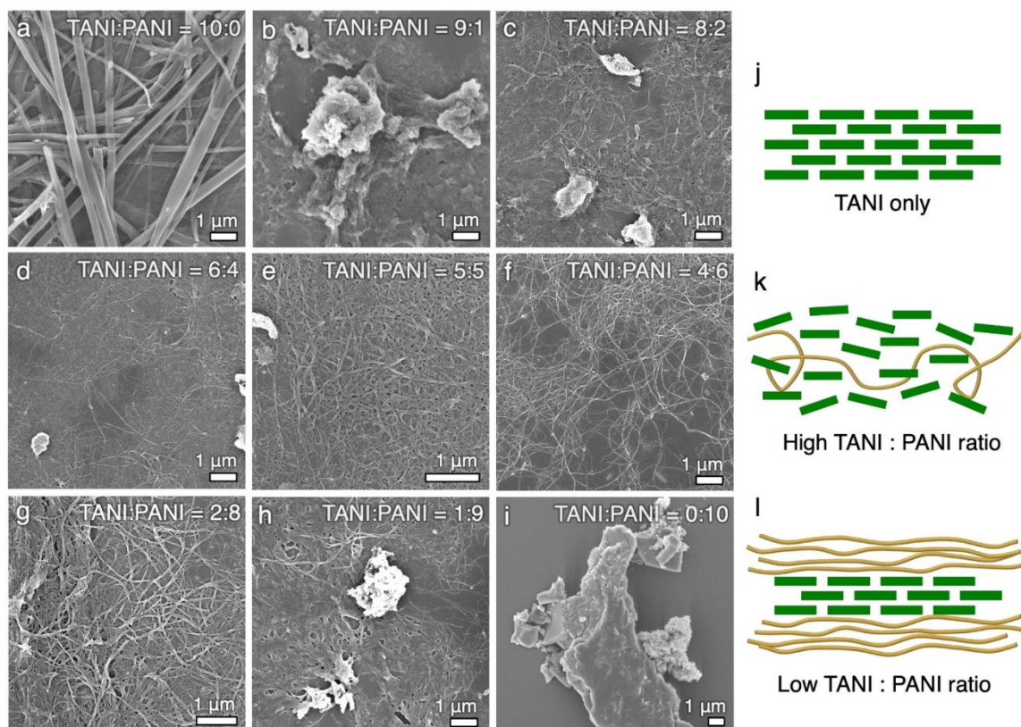
Fig. 2 (a)-(i) SEM images of TANI and TAS-PANI self-assembled at different TANI:PANI ratio in a solvent mixture of 20% THF and 80% 0.1 M \text{HClO}_4 . (j)-(l) Schematic diagrams illustrating the proposed mechanism behind the relationship between TANI:PANI ratio and the packing order.
