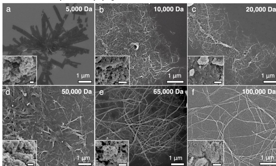
Fig. 3 SEM images of 20% TANI-assisted self-assembled nanostructures of PANI with defined molecular weight: (a) 5,000 Da, (b) 10,000 Da, (c) 20,000 Da, (d) 50,000 Da, (e) 65,000 Da, (f) 100,000 Da. The inset to each SEM shows PANI of the same molecular weight subjected to identical self-assembly environment in the absence of TANI. The scale bars in the insets are 1 \mu m.
