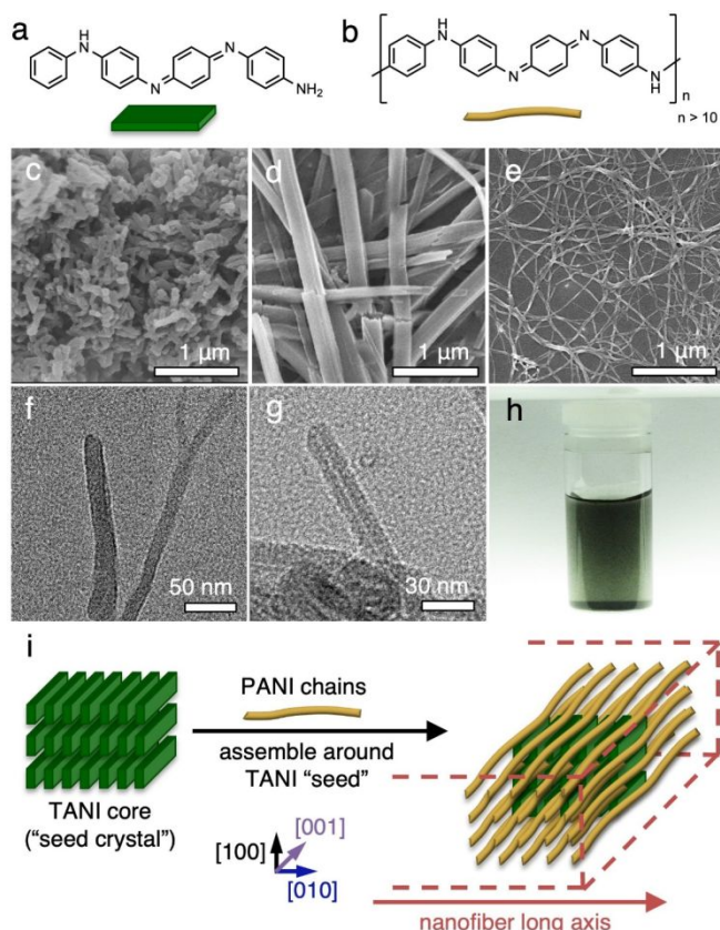
Fig. 1 Chemical structures of (a) tetraaniline and (b) polyaniline. (c)–(e) SEM images of (c) PANI nanofibers, (d) TANI nanowires, (e) self-assembled high aspect ratio PANI nanofibers containing 20% TANI (TAS-PANI). (f) TEM image of TAS-PANI. (g) TAS-PANI after acetone wash to remove TANI. (h) Photograph showing an aqueous dispersion of TAS-PANI. (i) Schematic diagram showing the mechanism behind TANI-assisted PANI assembly.
