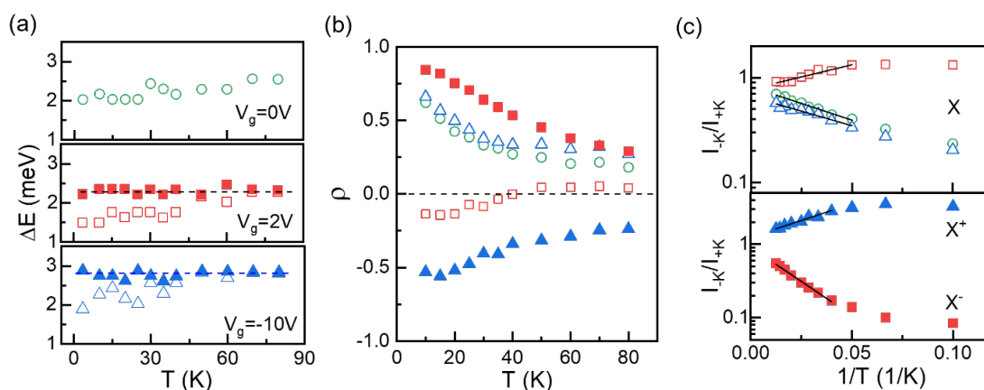
FIG. 4 Temperature dependency of repulsive polarons (open symbols) and attractive polarons (solid symbols) at V_g=0 (green), V_g=2V (red), and V_g=-10V (blue) for (a) polaron energy splitting, (b) valley polarization, and (c) intensity ratio of \sigma^- and \sigma^+ emission. Spectra were taken with linearly polarized excitation at 1.662 eV. In (c) the solid black lines are fits for extracting thermal activation energy.
