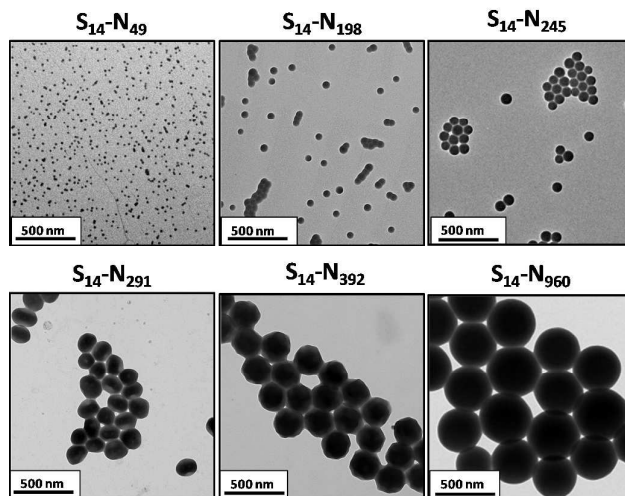
Figure 4. TEM images obtained for PSMA 14 -PNMEP x diblock copolymer nanoparticles prepared at 10% w/w solids in n -dodecane showing well-defined spherical nanoparticles (N.B. for brevity 'S' denotes PSMA and 'N' denotes PNMEP).
