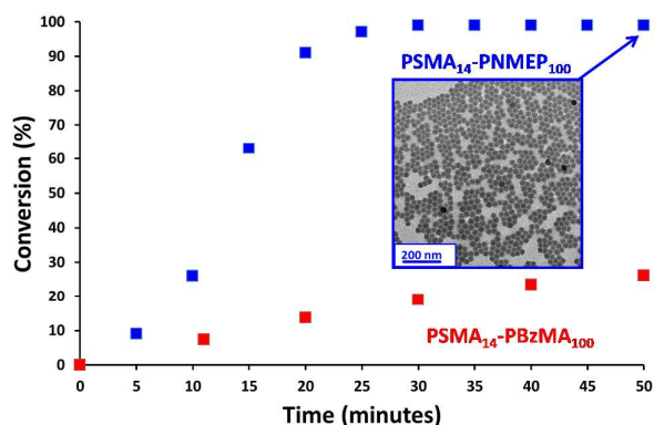
Figure 1. Kinetics of the polymerisation of NMEP and BzMA when targeting PSMA 14 -PNMEP 100 (blue) and PSMA 14 -PBzMA 100 (red) at 90 °C at 20% w/w solids. Insert: transmission electron microscopy image obtained after 50 min for PSMA 14 -PNMEP 100 showing the formation of near-monodisperse spherical nanoparticles with a mean diameter of 27 nm.
