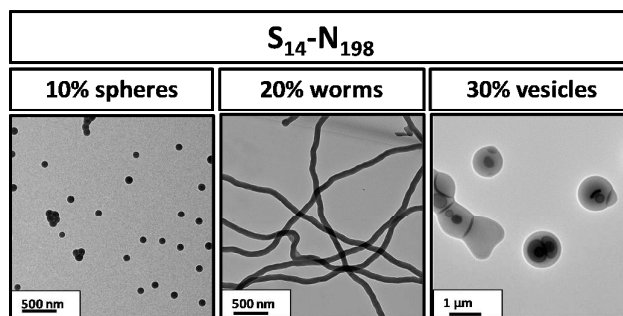
Figure 6. TEM images obtained for PSMA 14 -PNMEP 198 diblock copolymer nano-objects prepared at 10, 20 or 30% w/w solids confirming the formation of well-defined spheres, highly anisotropic worms and polydisperse vesicles, respectively (N.B. for brevity ‘S’ denotes PSMA and ‘N’ denotes PNMEP).
