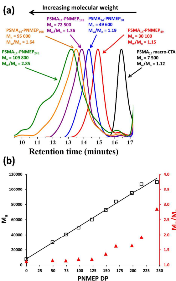
Figure 2. (a) 3:1 Chloroform/methanol GPC curves obtained for PSMA 14 -PNMEP x diblock copolymer nanoparticles prepared at 10% w/w solids via RAFT dispersion polymerisation of NMEP at 90 °C. (b) Relationship between target PNMEP DP and GPC M_n (black axis) and M_w/M_n (red axis) for the same series of PSMA 14 -PNMEP x diblock copolymer nanoparticles prepared at 10% w/w solids.
