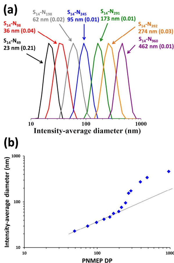
Figure 3. (a) DLS intensity-average size distributions for PSMA 14 -PNMEP x diblock copolymer nanoparticles prepared via RAFT dispersion polymerisation of NMEP at 10% w/w solids in n -dodecane at 90 °C (N.B. for brevity 'S' denotes PSMA and 'N' denotes PNMEP, the numbers in brackets refer to the DLS polydispersity in each case), (b) a plot of intensity-average diameter vs mean degree of polymerisation of the PNMEP core-forming block. TEM studies confirmed that spherical morphologies were obtained in all cases (see Figure 4).
