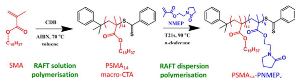
Scheme 1. (i) Synthesis of a PSMA 14 macro-CTA by RAFT solution polymerisation of SMA followed by (ii) the preparation of PSMA 14 -PNMEP x nano-objects via RAFT dispersion polymerisation of NMEP in n -dodecane.
