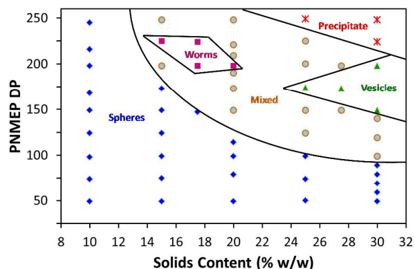
Figure 5. Phase diagram for a series of PSMA 14 -PNMEP x diblock copolymers synthesised by RAFT dispersion polymerisation in n -dodecane at various concentrations ranging between 10 and 30% w/w. Post-polymerisation analysis of each diblock copolymer dispersion by TEM determined the phase boundaries.
