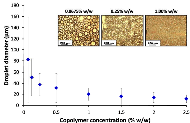
Figure 8. Concentration dependence of the mean volume-average droplet diameter (as determined by laser diffraction) for oil-in-water Pickering emulsions prepared at a constant shear rate of 13,200 rpm using PSMA 14 -PNMEP 49 spheres. The error bars shown represent the standard deviation of each mean volume-average droplet diameter, rather than the experimental error. Inset: optical microscopy images of the droplets prepared at 0.0675, 0.25 and 1.00% w/w. Scale bar = 200 µm.
