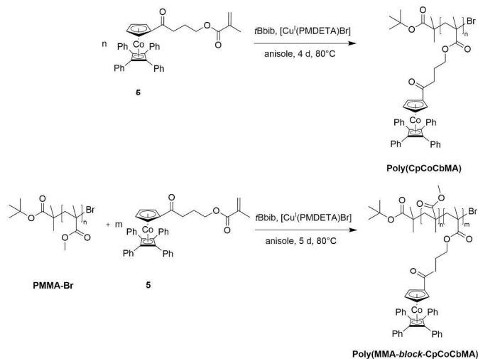
Fig. 4 Atom Transfer Radical Polymerization (ATRP) of CpCoCbMA 5 (top) and block copolymerization starting with an PMMA-Br macro-initiator (bottom) for the preparation of PMMA- block -P(CpCoCbMA).
