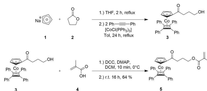
Fig. 2 One-pot synthesis of ( \eta^5 -cyclopentadienyl-4-hydroxybutan-1-on)cobalt( \eta^4 -tetraphenyl-cyclobutadiene) 3 (CpCoCb) by sequential addition of given reagents (top, see Experimental Section). Steglich esterification of CpCoCb 3 with methacrylic acid 4 yielded the cobalt-methacrylate monomer 5 CpCoCbMA.
