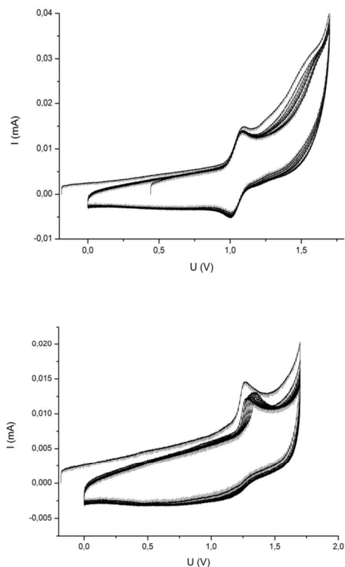
Fig. 9: Repeated cyclic voltammetry curves (10 cycles) of CpCoCbMA monomer (top) and poly(CpCoCbMA) (bottom) in CH 2 Cl 2 with TBAHFP (0.1 M) as electrolyte. Scan rate was 20 mV s -1 .
