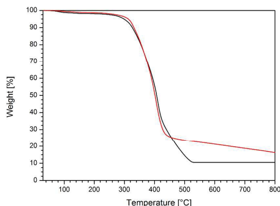
Fig. 6 TGA curves of poly(CpCoCbMA) performed with a heat rate of 10 \text{ K min}^{-1} to 800^\circ\text{C} in an oxygen (black curve) and nitrogen (red curve) atmosphere.
