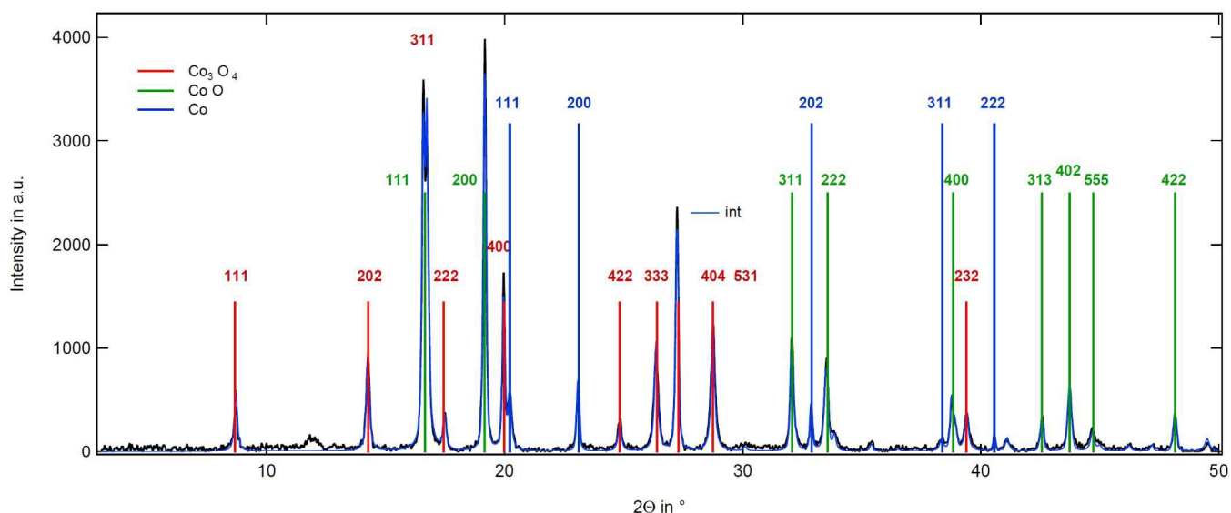
Fig. 7 XRD pattern on the magnetic material obtained by thermal treatment of poly(CpCoCbMA) samples in nitrogen atmosphere at 800°C (see text).
