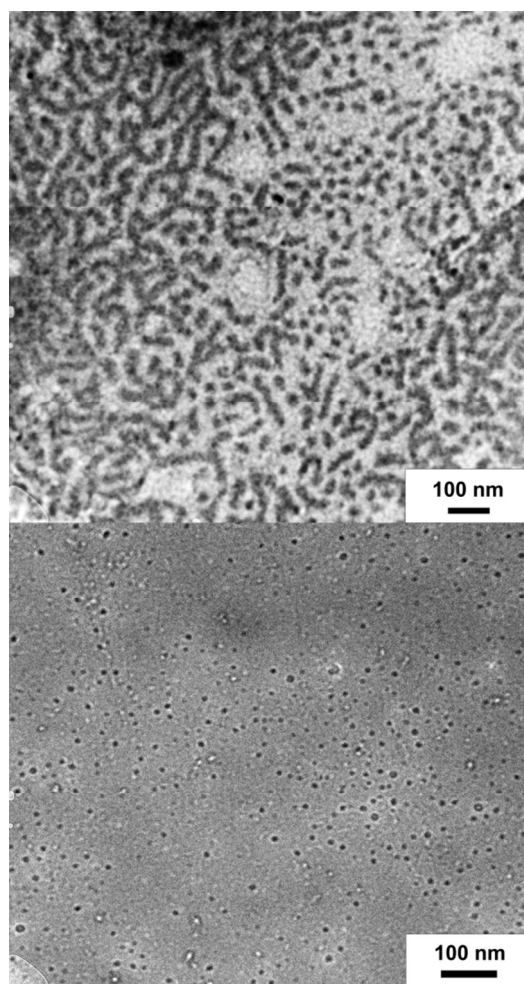
Fig. 10 TEM images of PMMA- block -PCpCoCbMA micelles formed in chloroform after treatment with decamethylcobaltocene (Cp* 2 Co) (top) or treatment with NOBF 4 (bottom). The micelles were deposited on a carbon-coated copper grid followed by drying at ambient temperature. Scale bars correspond to 100 nm.
