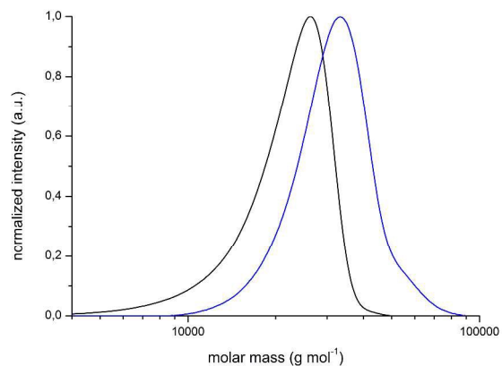
Fig. 5 Molecular weight distribution of poly(MMA- b -lock-CpCoCbMA) in THF (blue curve) obtained by sequential ATRP of the PMMA-Br macro-initiator (black curve) with CpCoCbMA 5 . Obtained values were calibrated against PS standards.
