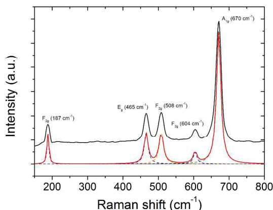
Fig. 8 Raman spectrum of the sample prepared upon pyrolysis of poly(CpCoCbMA) at 800°C in nitrogen atmosphere showing the five Raman-active optical-phonon modes of spinel-type \text{Co}_3\text{O}_4 .
