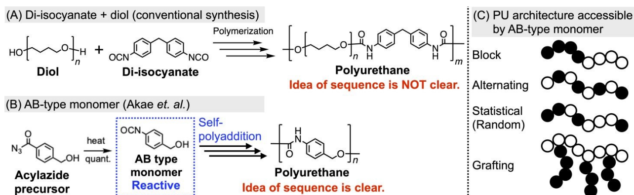
Figure 1. General concept of this work as illustrated using PU as a model system; (A) PU synthesis by the conventional method; (B) PU synthesis based on the AB-type monomer featuring both acylazide and alcohol groups; [69-73] (C) PU architectures accessible by AB-type monomer.
