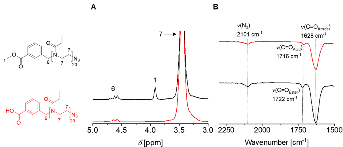
Fig. 5 Spectroscopic confirmation of end groups in the heterotelechelic 3M-EtOx 20 -N 3 (black) and 3A-EtOx 20 -N 3 (red). (A) Overlay of ^1\text{H} NMR spectra ( \text{CDCl}_3 , 300 MHz). (B) Overlay of IR spectra with assignment of characteristic vibrational bands. Full spectra are shown in the SI.
