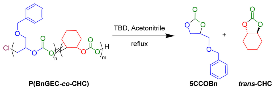
Scheme 3 Depolymerization of \text{P}(\text{BnGEC-co-CHC}) terpolymer using 1,5,7-triazabicyclo[4.4.0]dec-5-ene (TBD).
