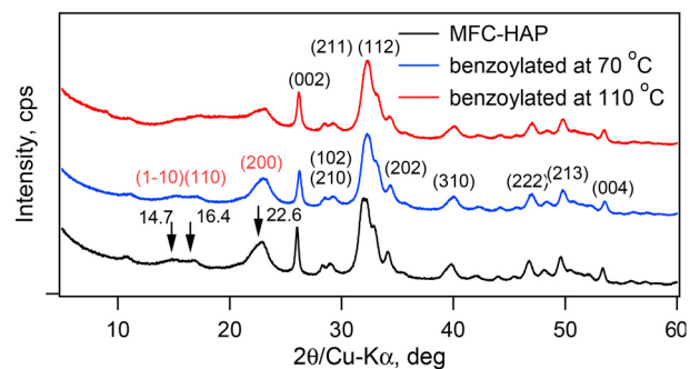
Fig. 3 XRD patterns of the parent MFC–HAP composite and the benzoylated MFC–HAP composites. The indices of the diffraction peaks of HAP and those of cellulose I β are shown in black and red, respectively.
