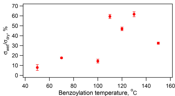
Fig. 8 Plot of the ratios of bending strengths of the wet compacts to those of the dry compacts ( \sigma_{wet}/\sigma_{dry} ) against benzoylation temperatures. The standard errors obtained from three to four measurements were represented by error bars.
